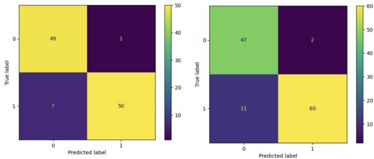
Figure 17: Isolation forest
