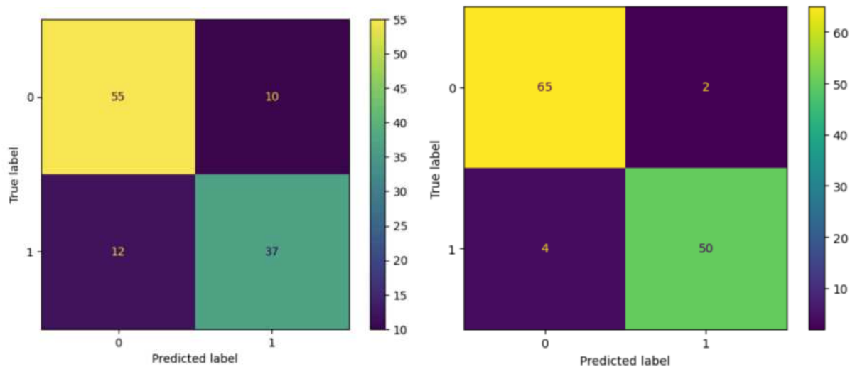
Figure 14: Isolation forest
