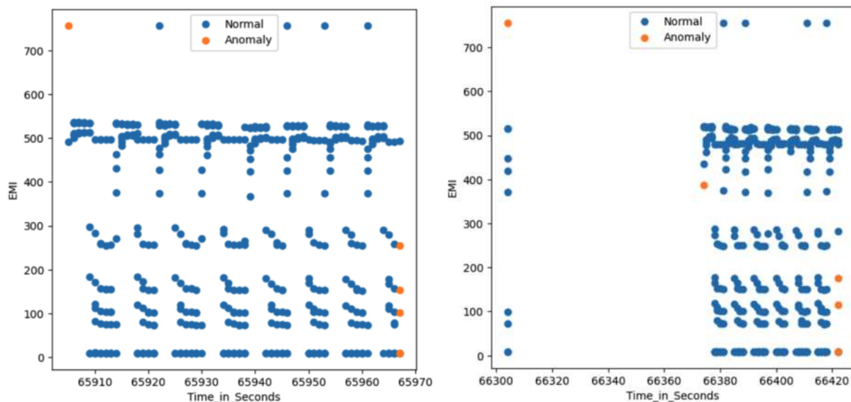
Figure 20: Isolation forest
