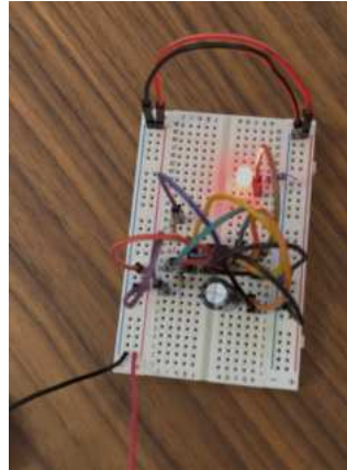
Figure 2: Astable 555 timer
