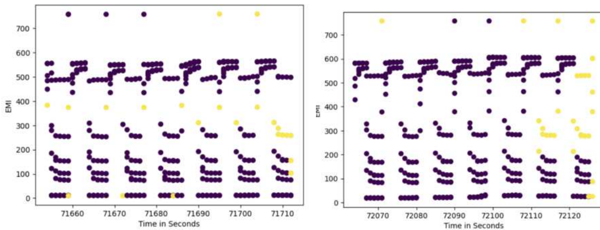
Figure 15: Random forest
