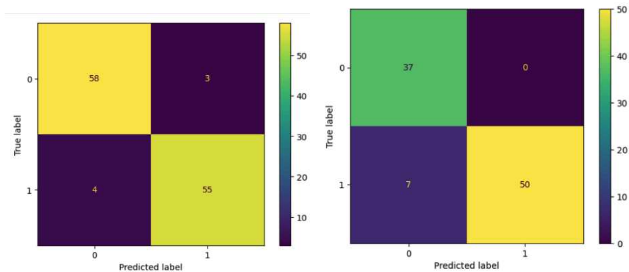
Figure 20: Isolation forest
